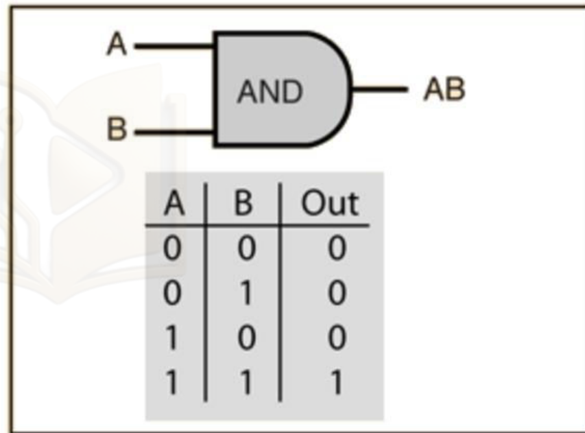
AND Gate
